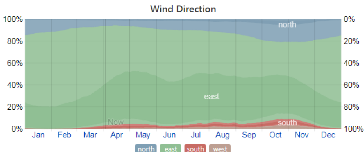
Figure 8: Percentage of hours in which the mean wind direction is from each of the four cardinal wind directions, excluding hours in which the mean wind speed is less than 1.0 mph
