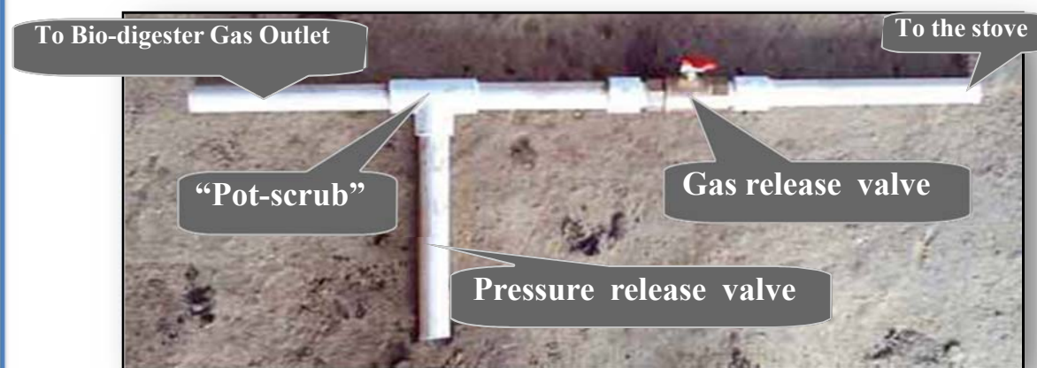
Fig 9: Completed Valve Assembly
