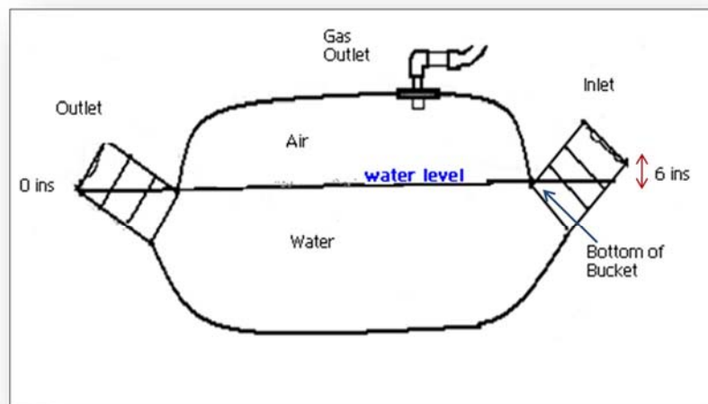
Fig 13: Inlet and Outlet Positioning
