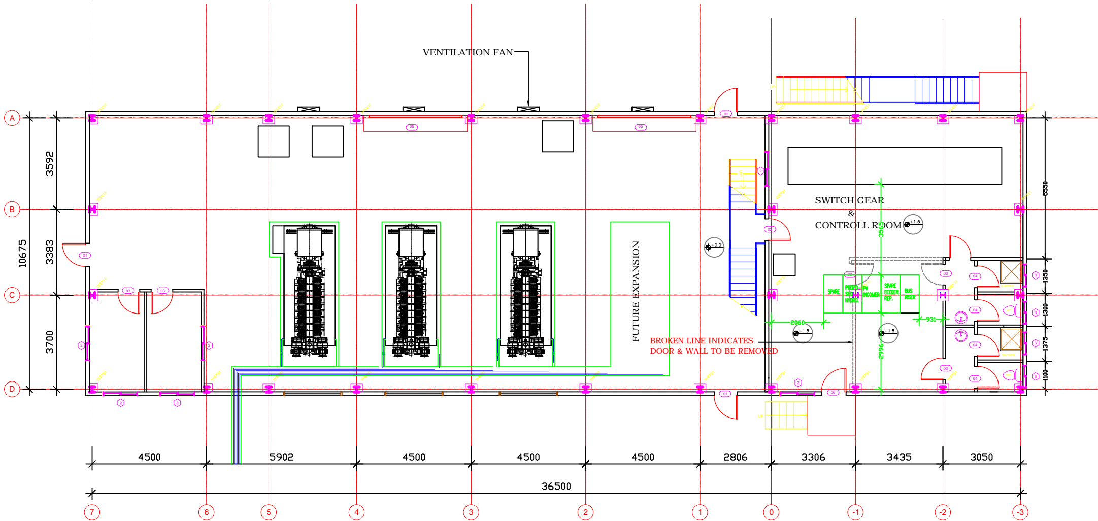
GROUND FLOOR POWER PLANT SCALE: 1:50
